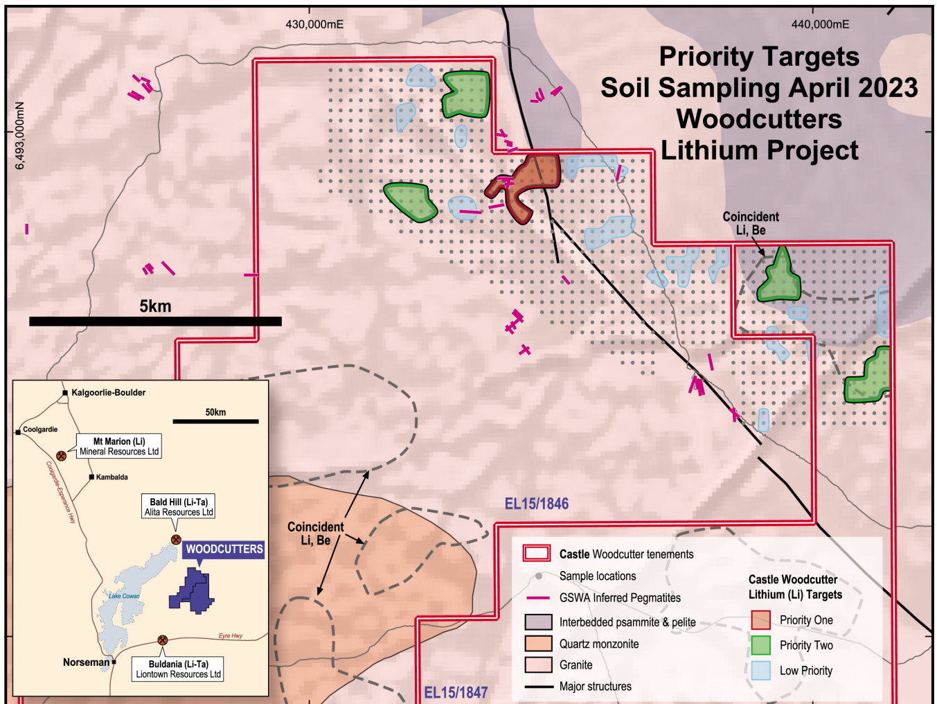
Fig 1: Woodcutters Lithium Project: Location of priority lithium-in-soil anomalies defined by Castle’s recent sampling and several historical anomalies defined by an analysis of an historical third-party sampling dataset.
